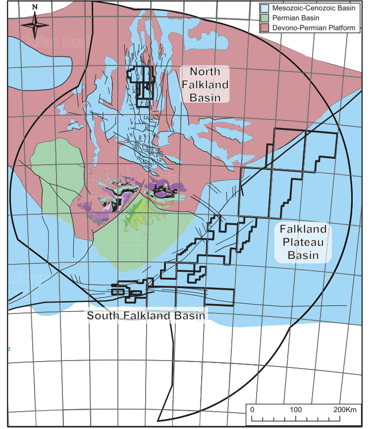
Map illustrating the regional geology of the Falkland Islands and the offshore basins.
